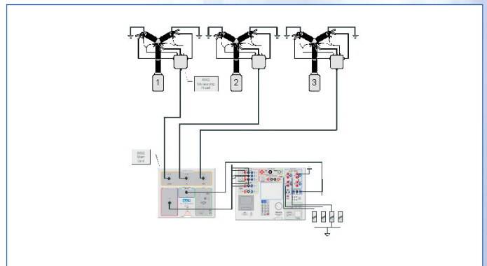
BSG-1000 Connection Scheme
